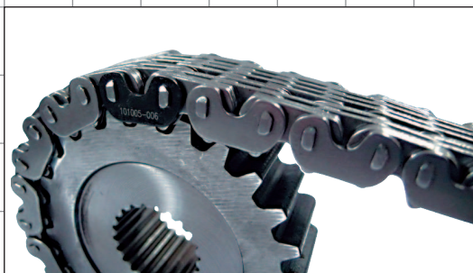
Rocker joint type silent chains
